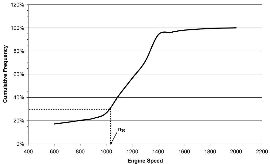
Figure 2: Example Not-To-Exceed Control Area When C Speed < 2,400 rpm
